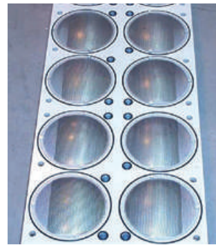
Distribution Manifold
